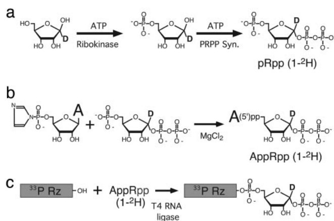
Fig. 2. The synthesis of the ( ^{33}\text{P} , 1\text{-}^2\text{H} ) dual-labeled ribozyme-PRPP species. (a) Ribose isotopically substituted with 1\text{-}^2\text{H} was converted first to ribose 5-phosphate and then PRPP by using ribokinase and PRPP synthase successively in the presence of ATP. (b) PRPP purified by using a DEAE column was reacted with adenosine-5'-phosphorimidazole (19) to synthesize adenylylated PRPP (AppRpp), which was purified by reverse-phase HPLC. (c) Ribozyme (Rz) radiolabeled during T7 transcription with ^{33}\text{P} was covalently attached at its 3' end to the isotopically modified PRPP by using T4 RNA ligase.
