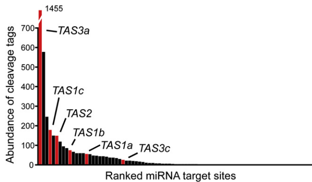
Figure 3. High Accumulation Levels of TAS Cleavage Products
